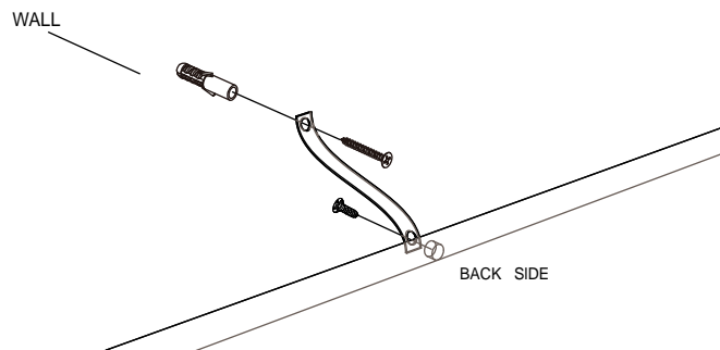
Anti-tit Strap X1
